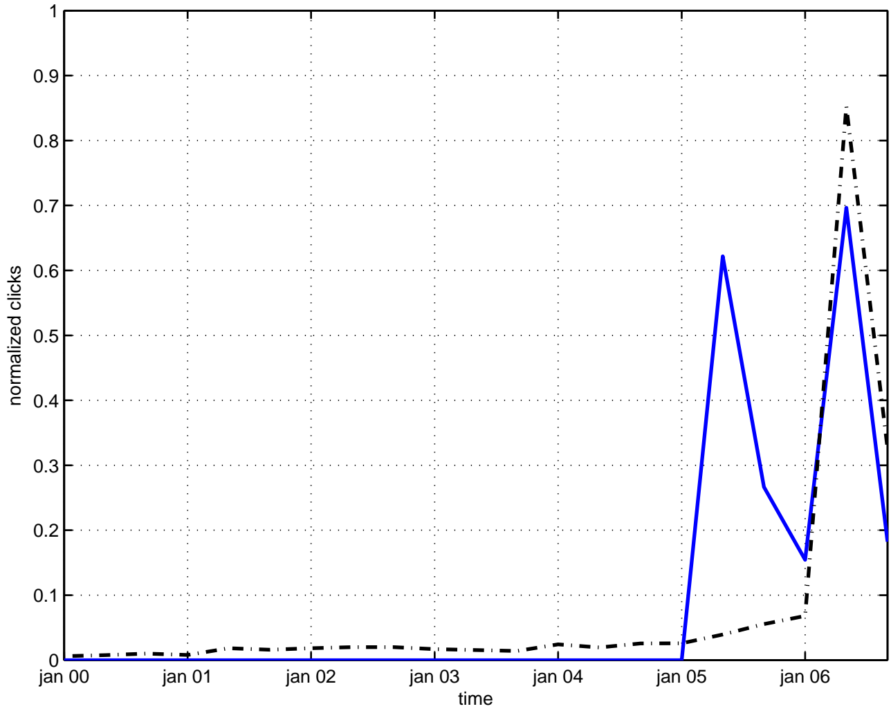
mass nucleon
