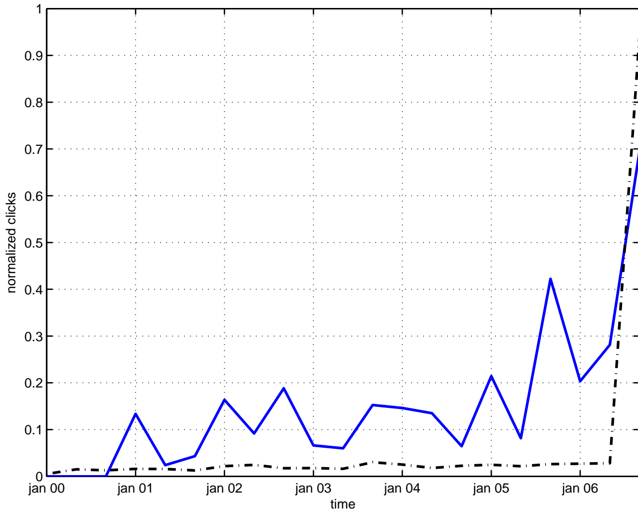
mass neutrino
