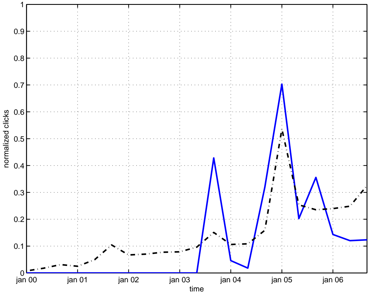
mass inflaton
