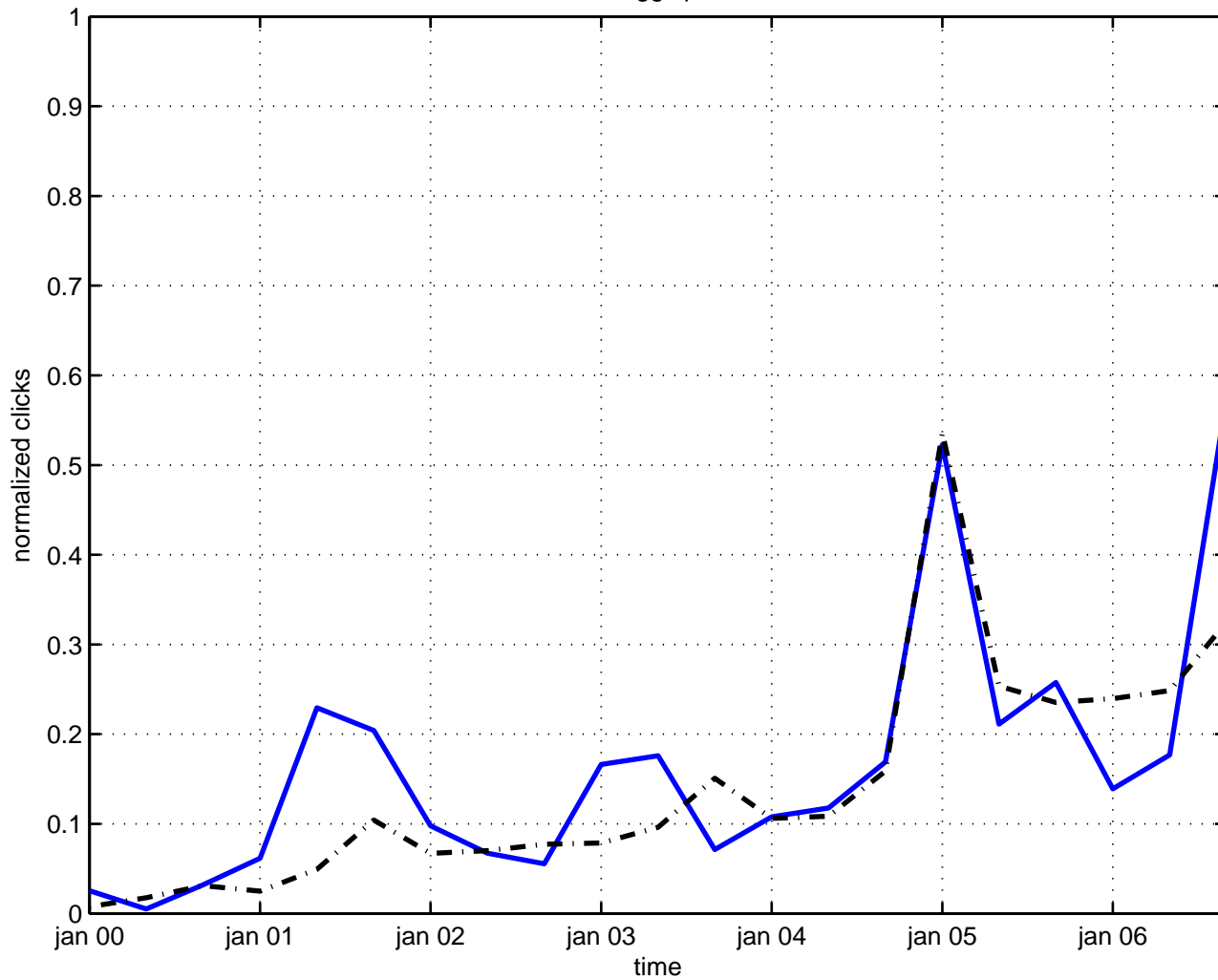
mass higgs particle
