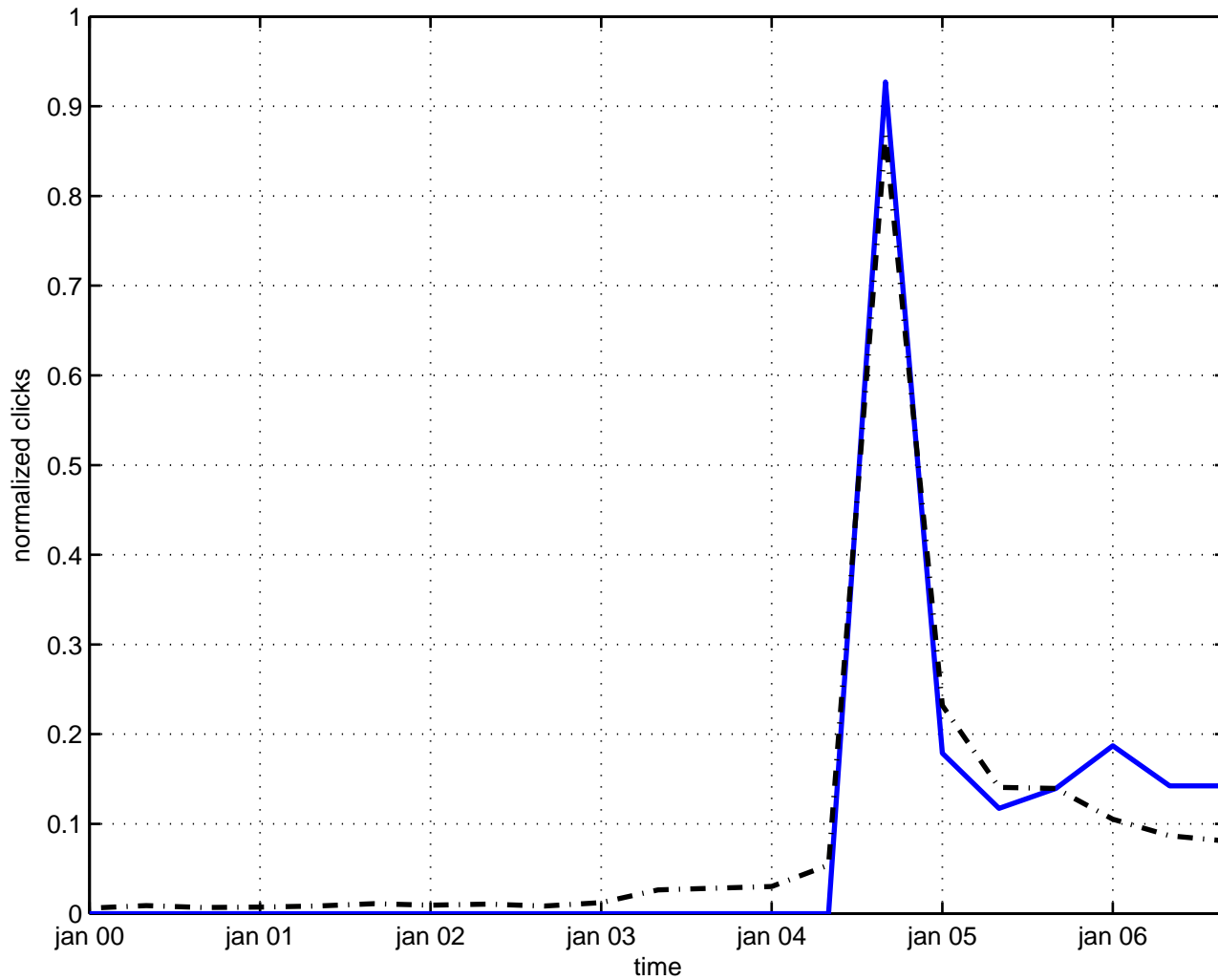
mass hadron
