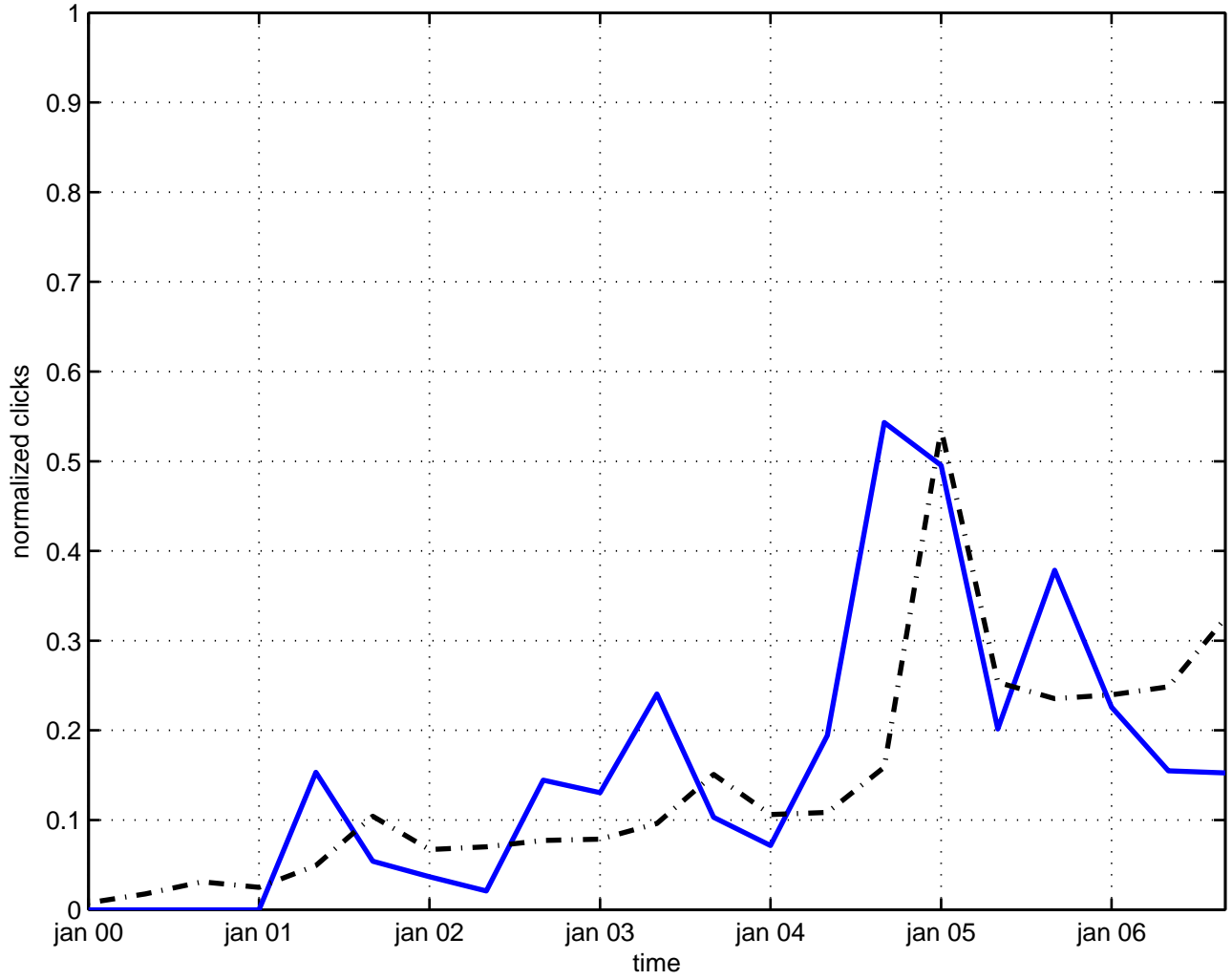
mass graviton
