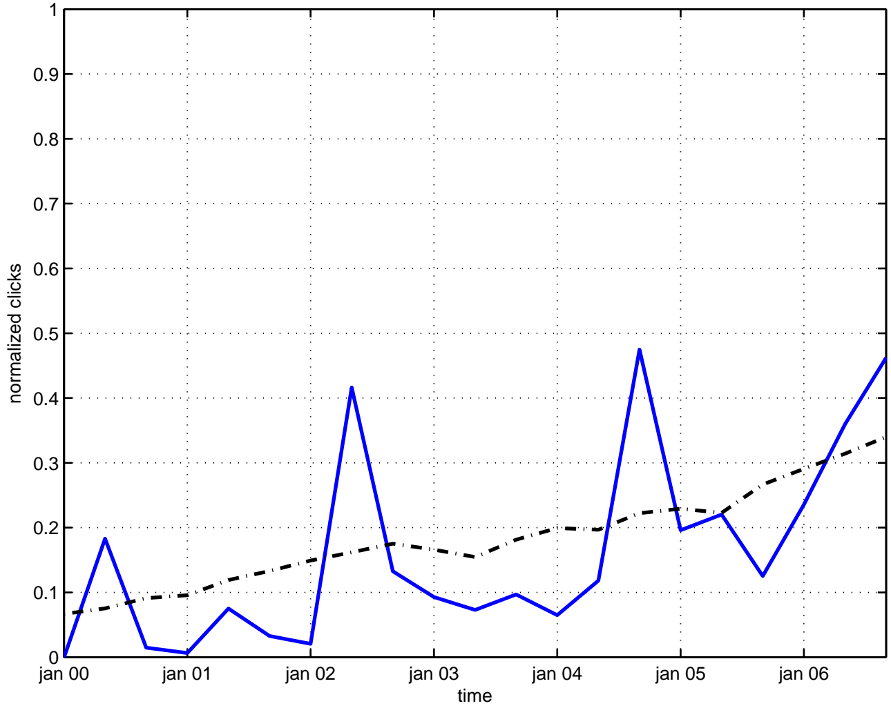
mass gravitino
