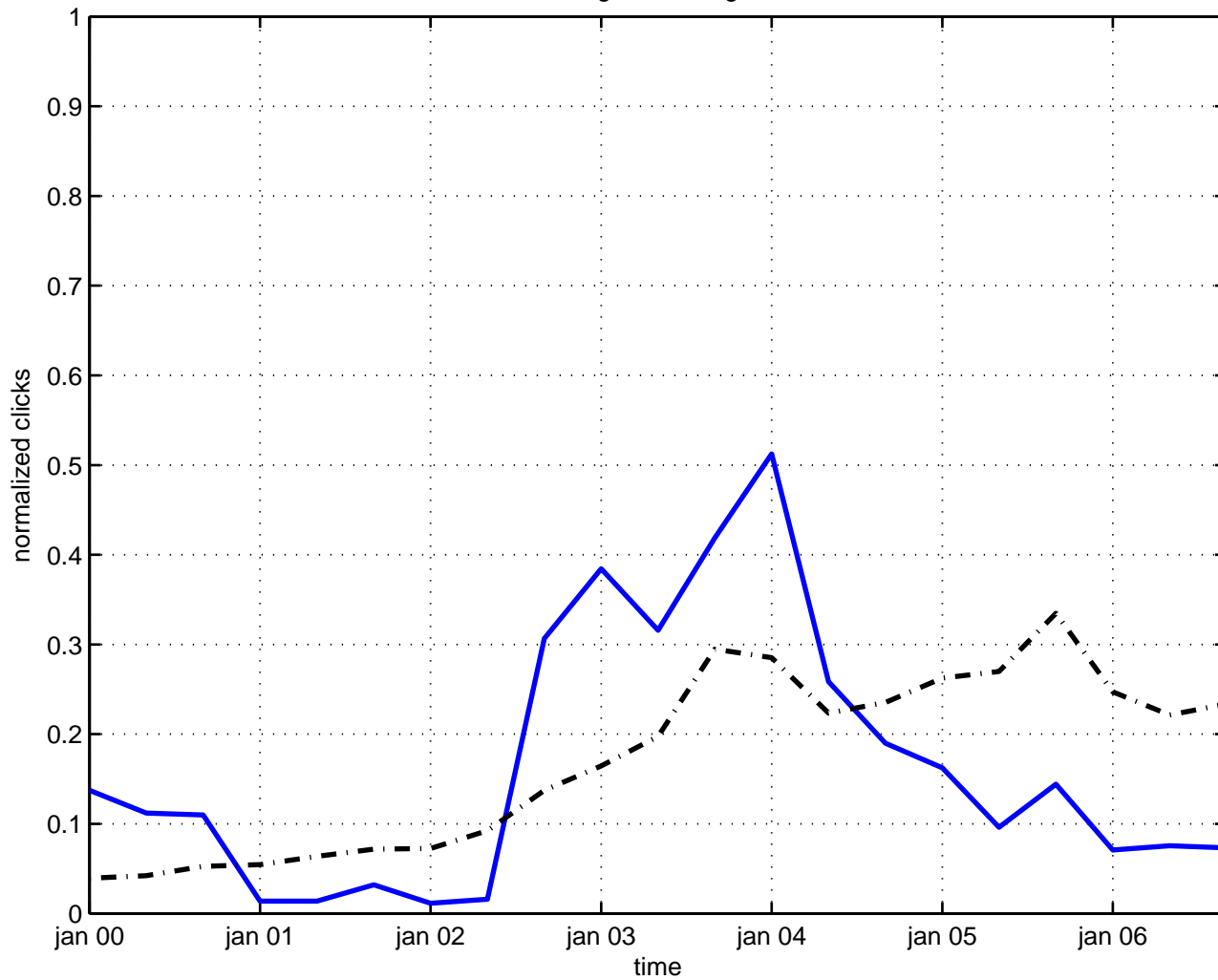
mass generation gluon
