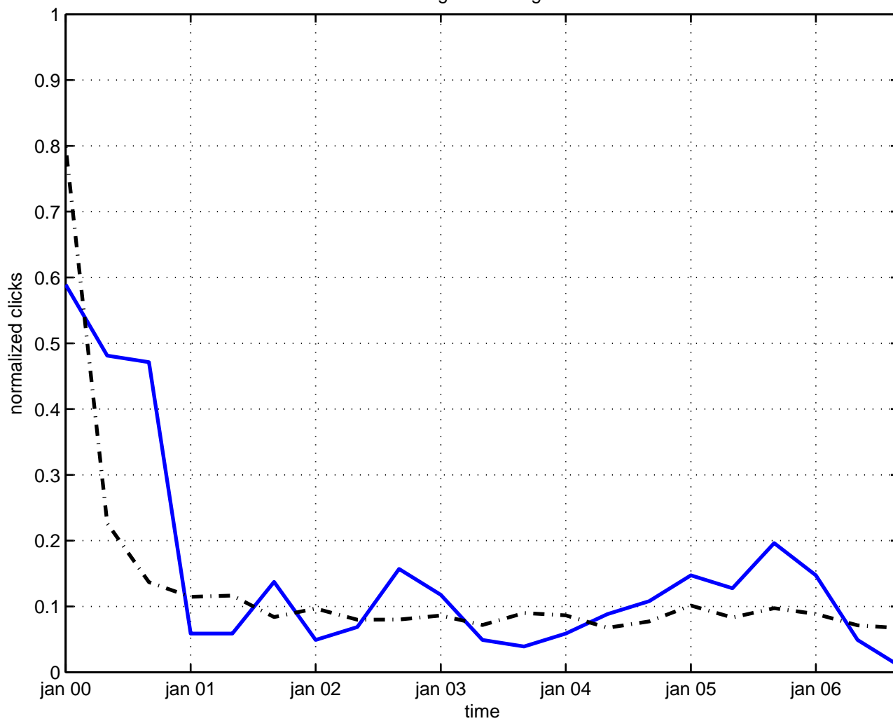
mass generation ghost
