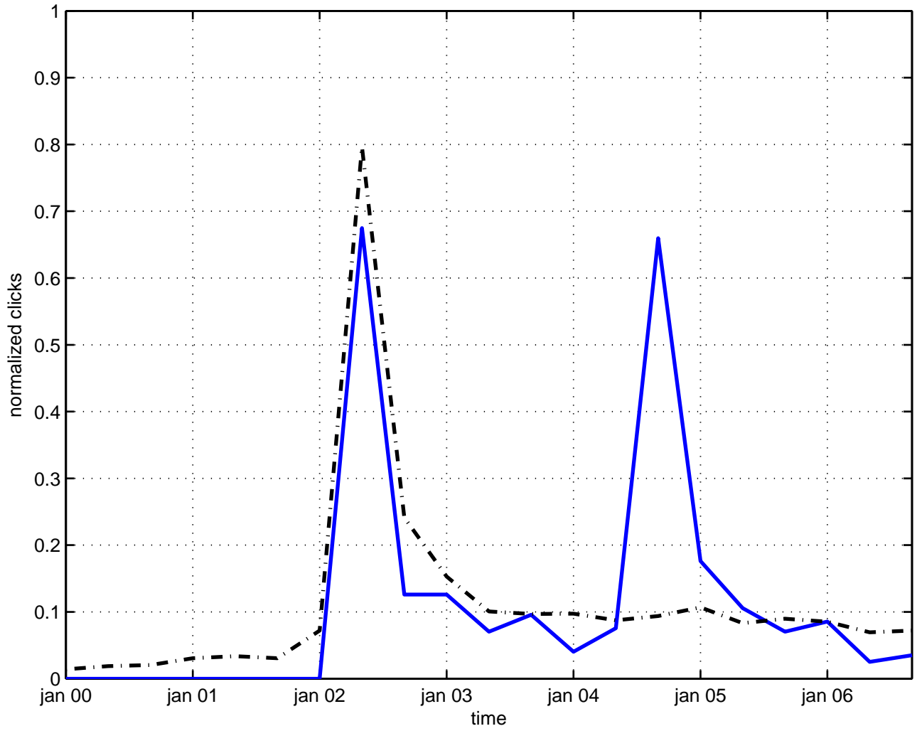
mass dyon
