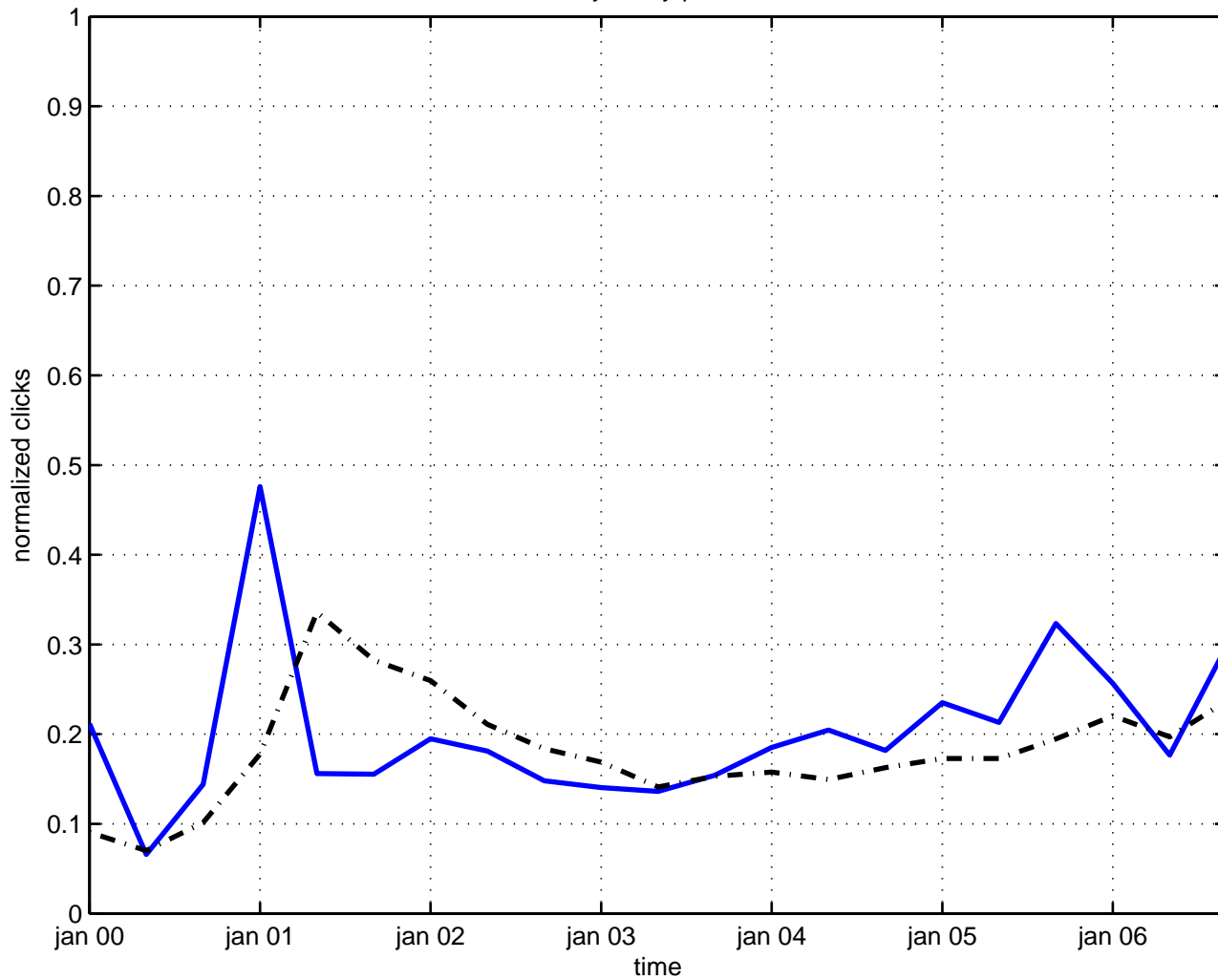
many-body problem
