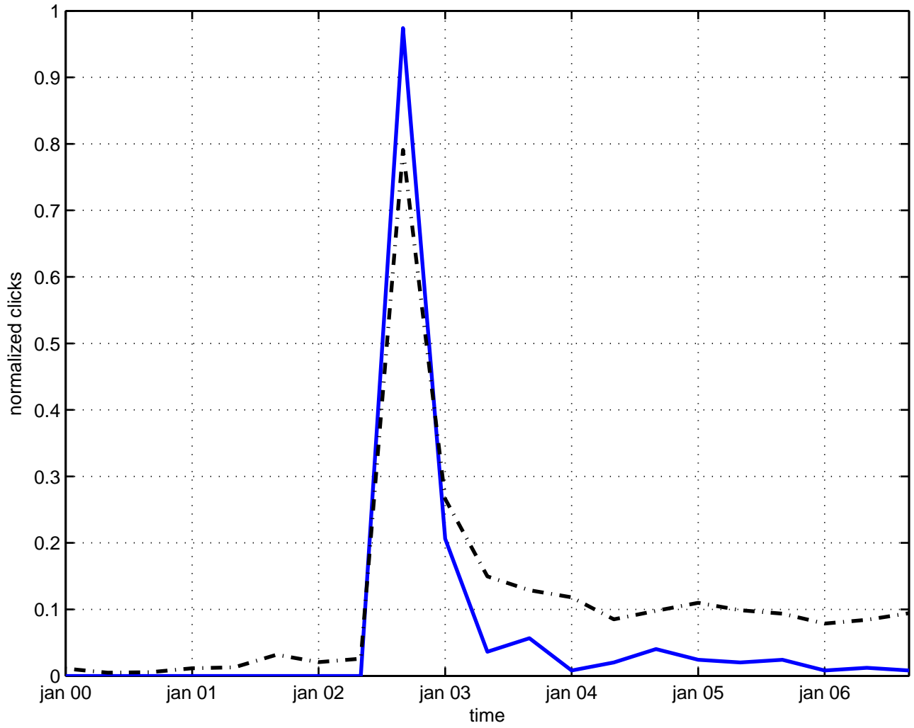
majorana vector
