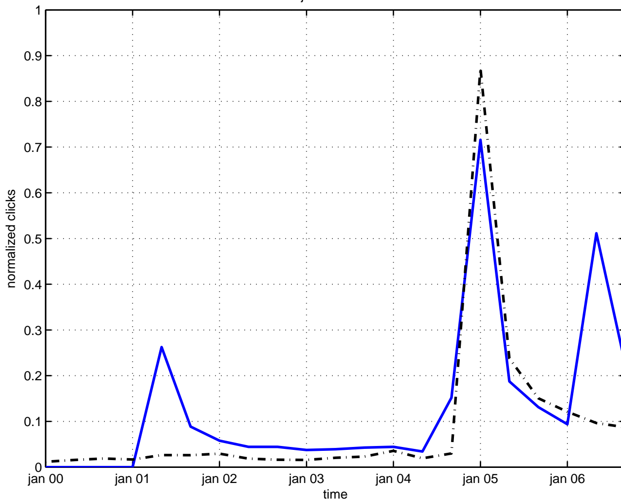
majorana neutrino
