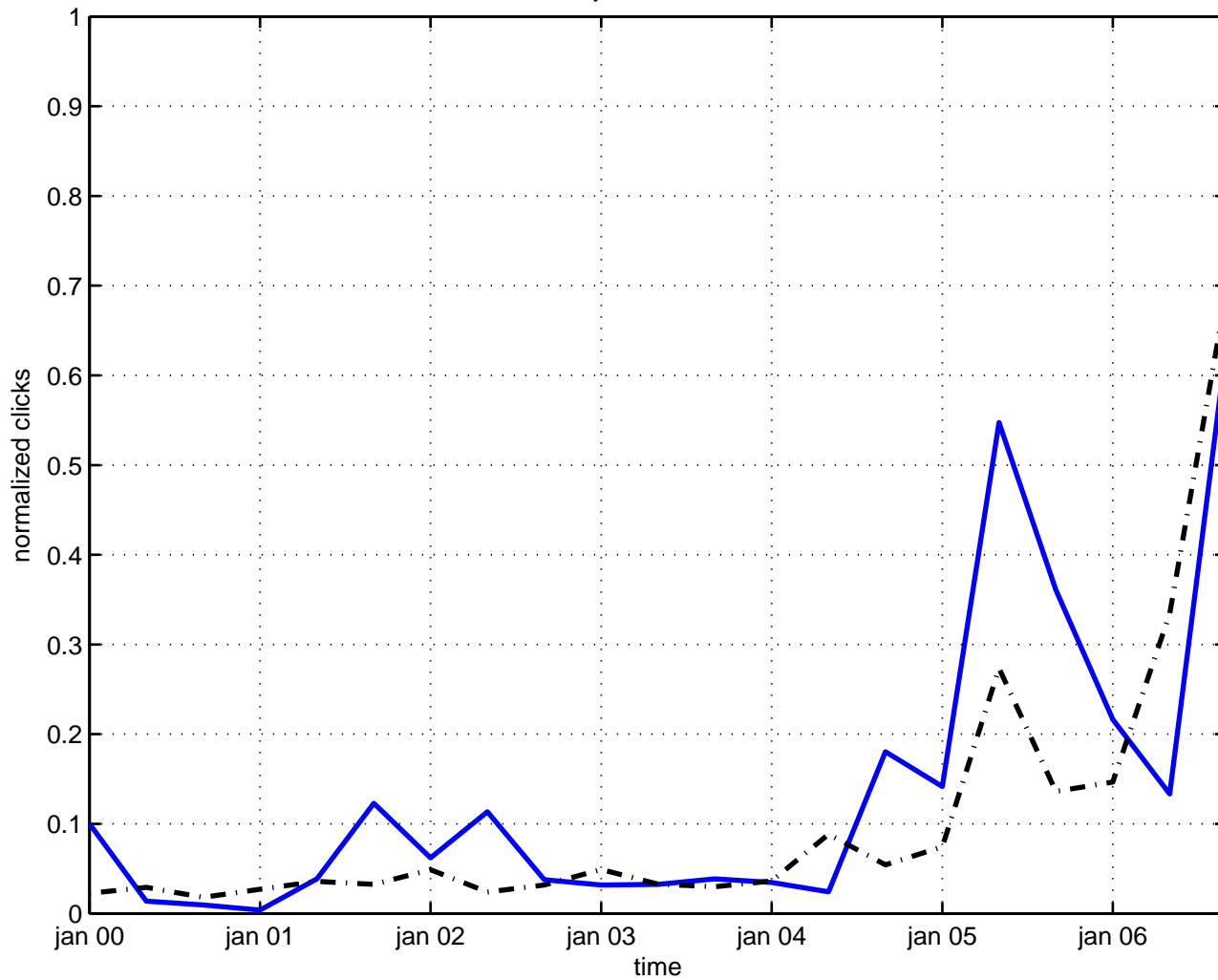
majorana fermion
