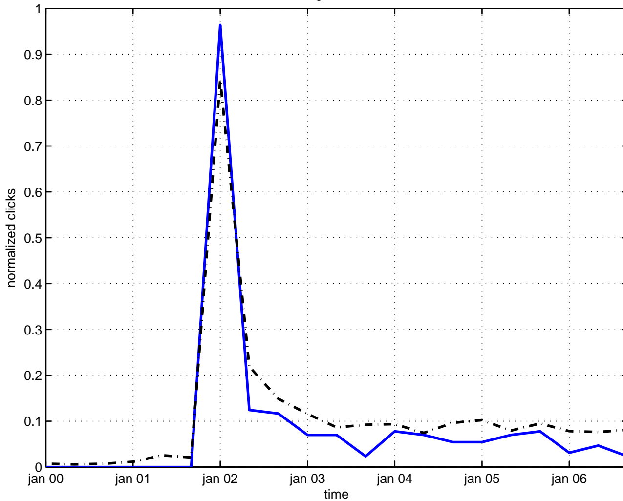
magnus force
