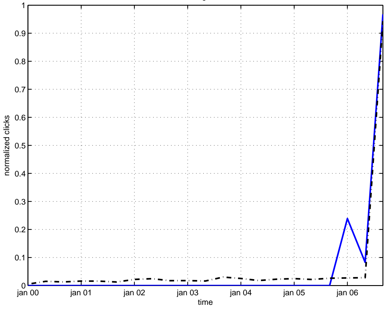
magnon
