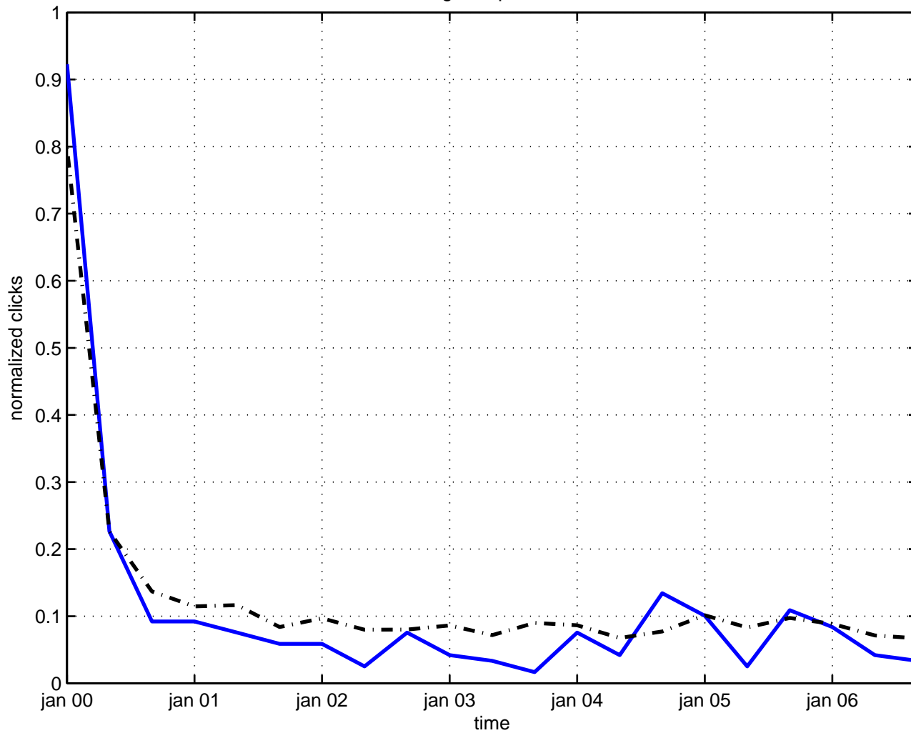
magnetic p-brane
