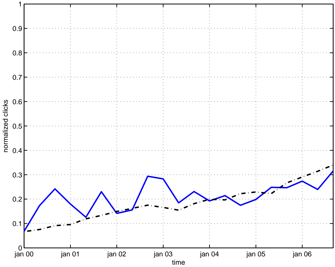
magnetic monopole
