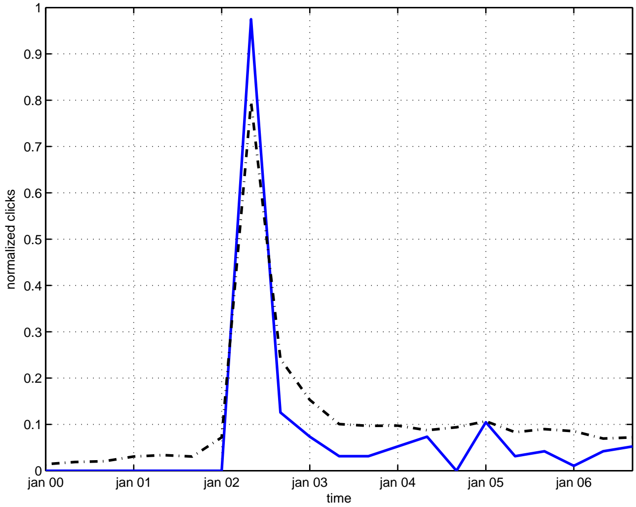
magnetic monopole gravitation
