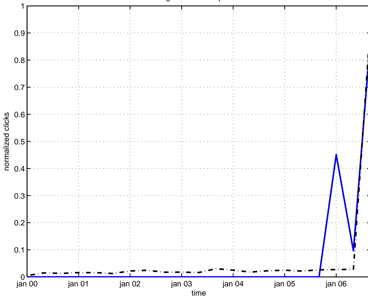
magnetic moment photon
