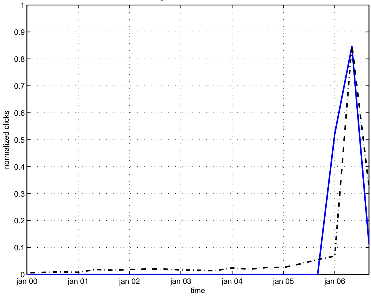
magnetic moment black hole
