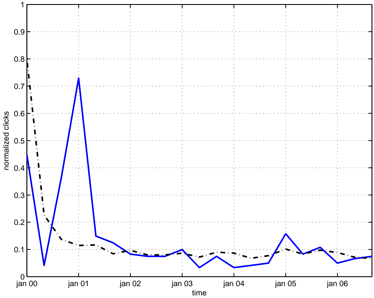
magnetic catalysis
