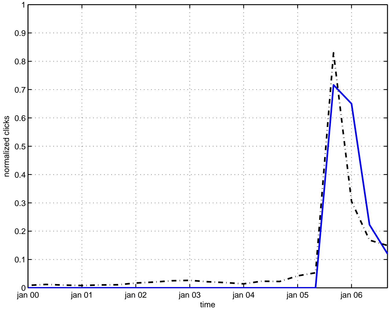
magnetic bag model
