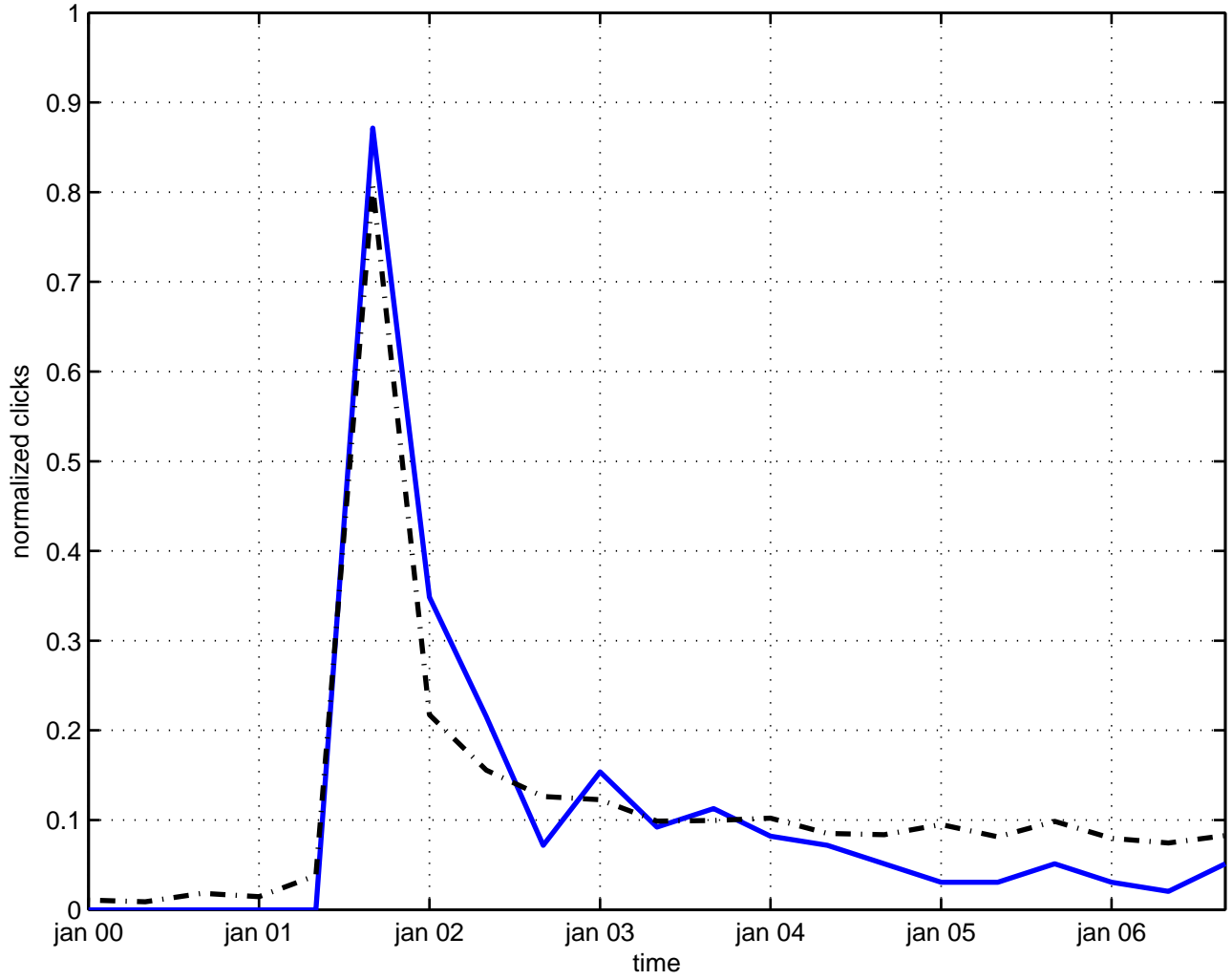
m(3) x s(1) space-time
