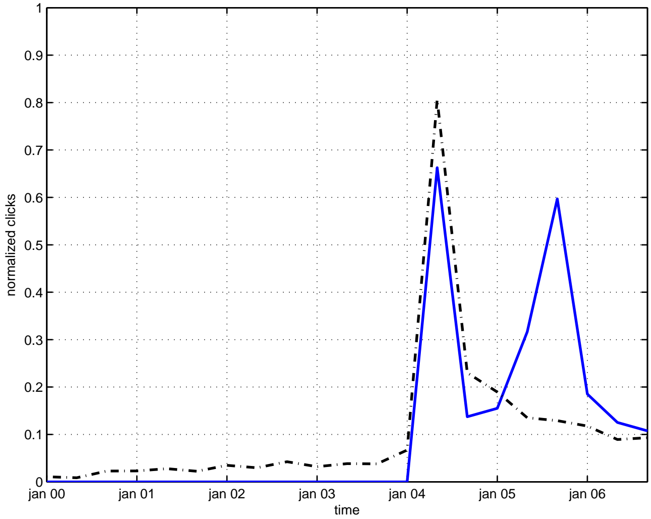
lyapunov exponent
