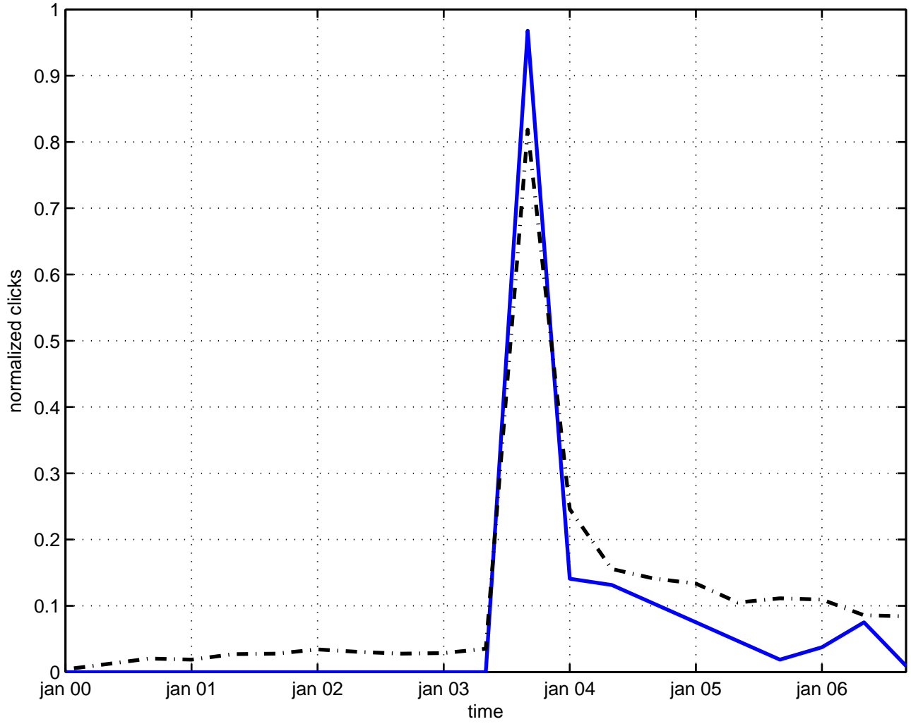
luttinger liquid
