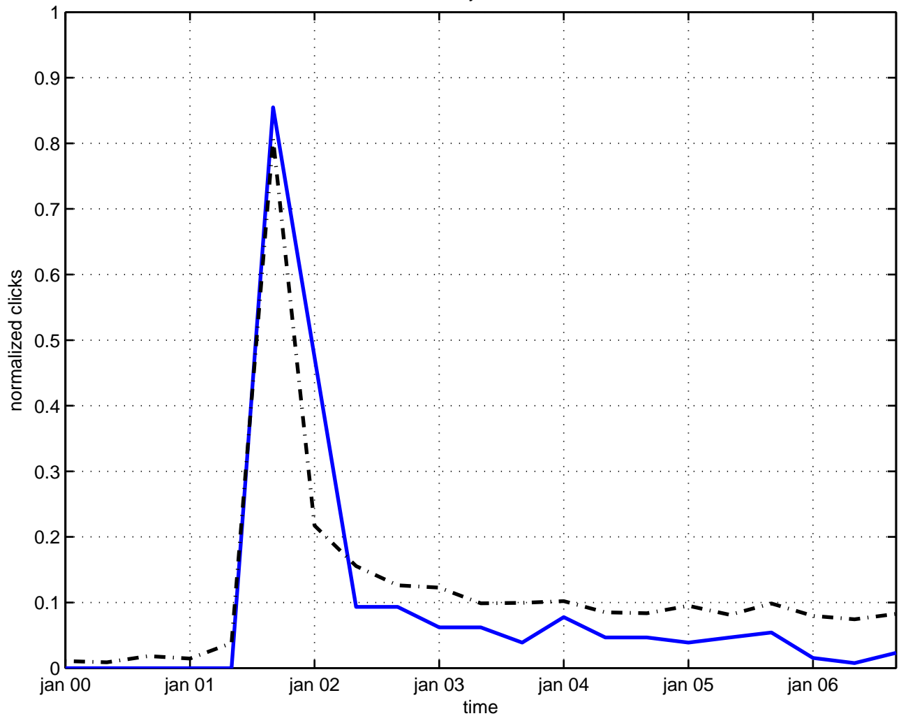
luminosity black hole
