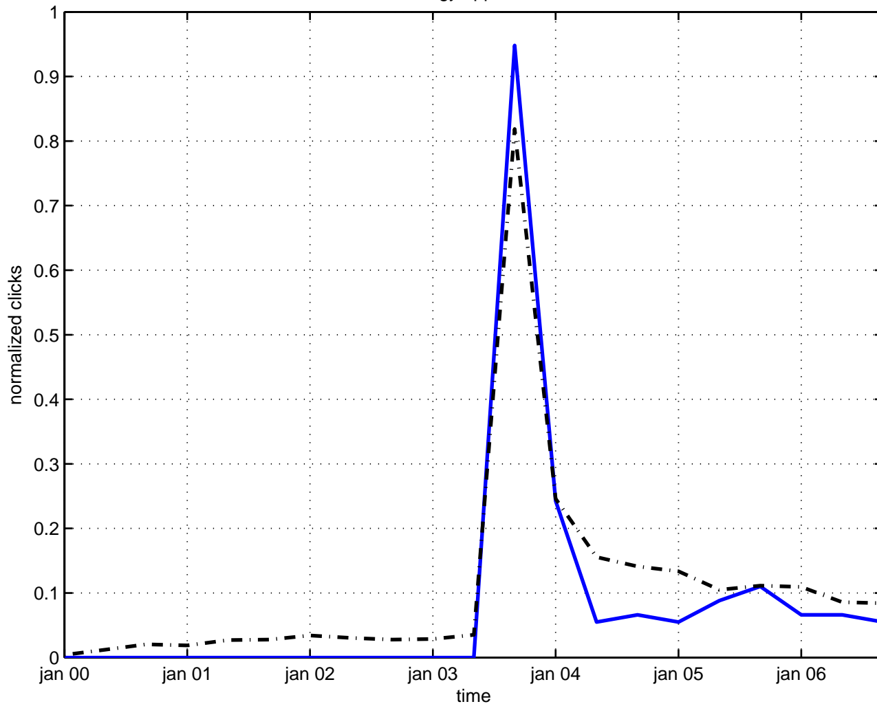
low energy approximation
