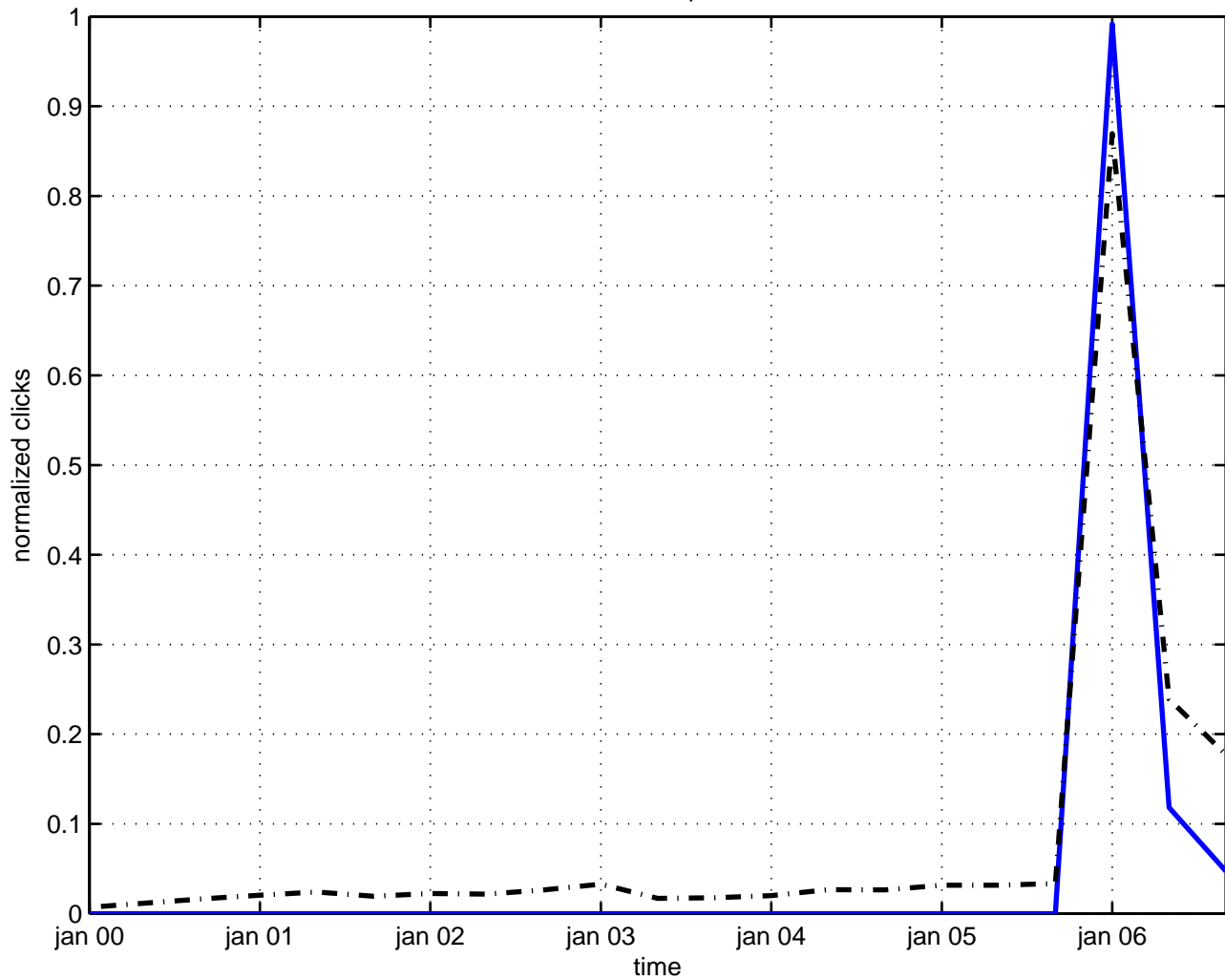
lorentz spin
