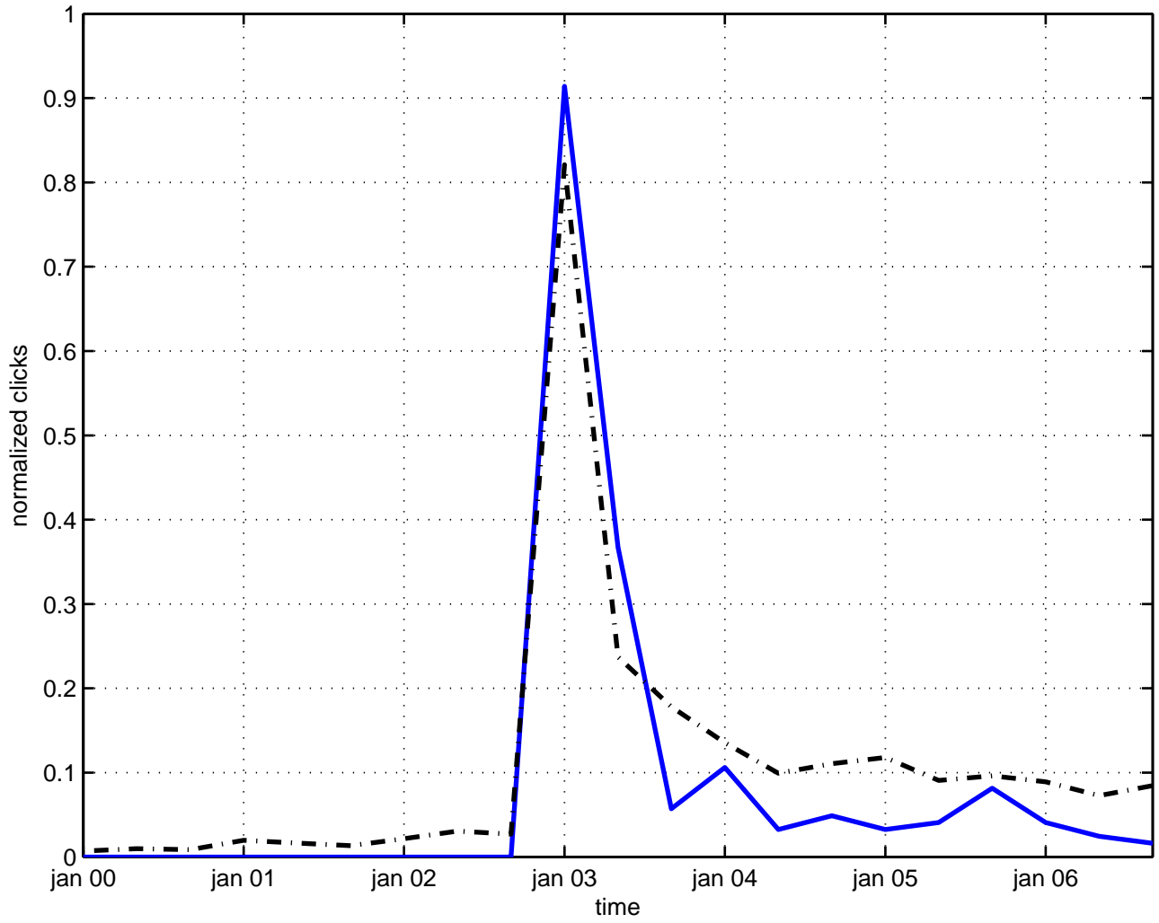
lorentz anomaly
