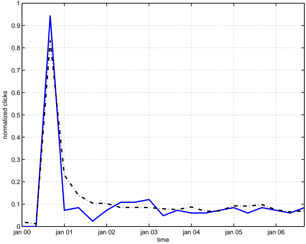
loop space algebra
