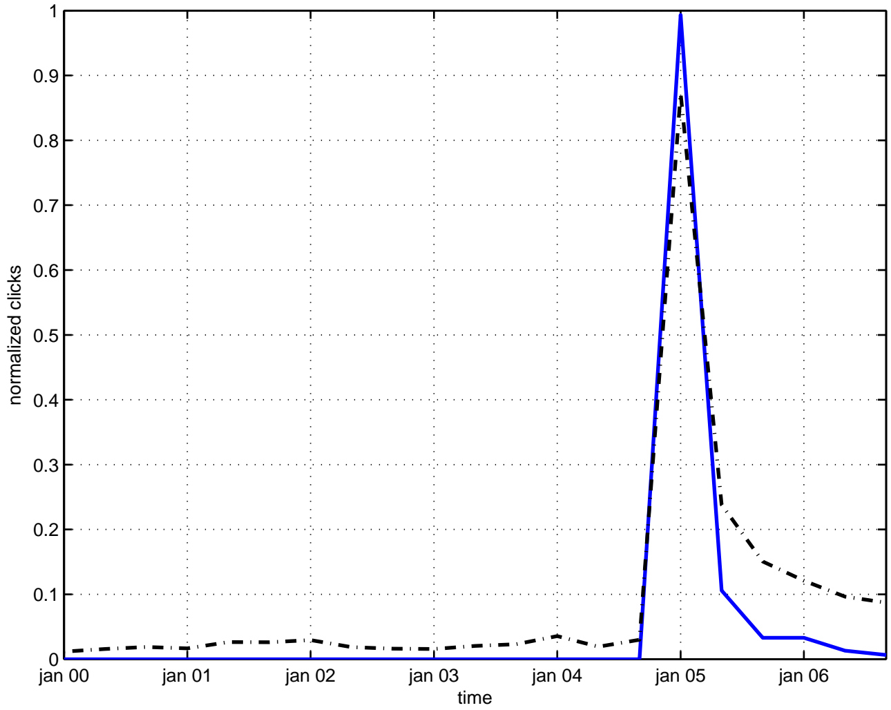
long-range gravitation
