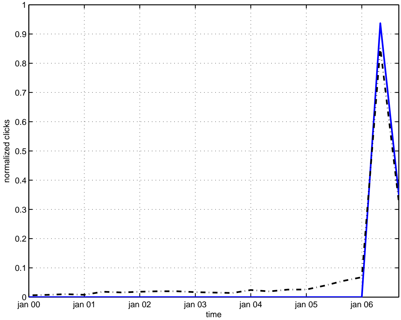
localization space-time
