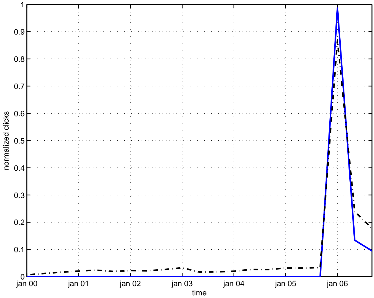
localization partition function
