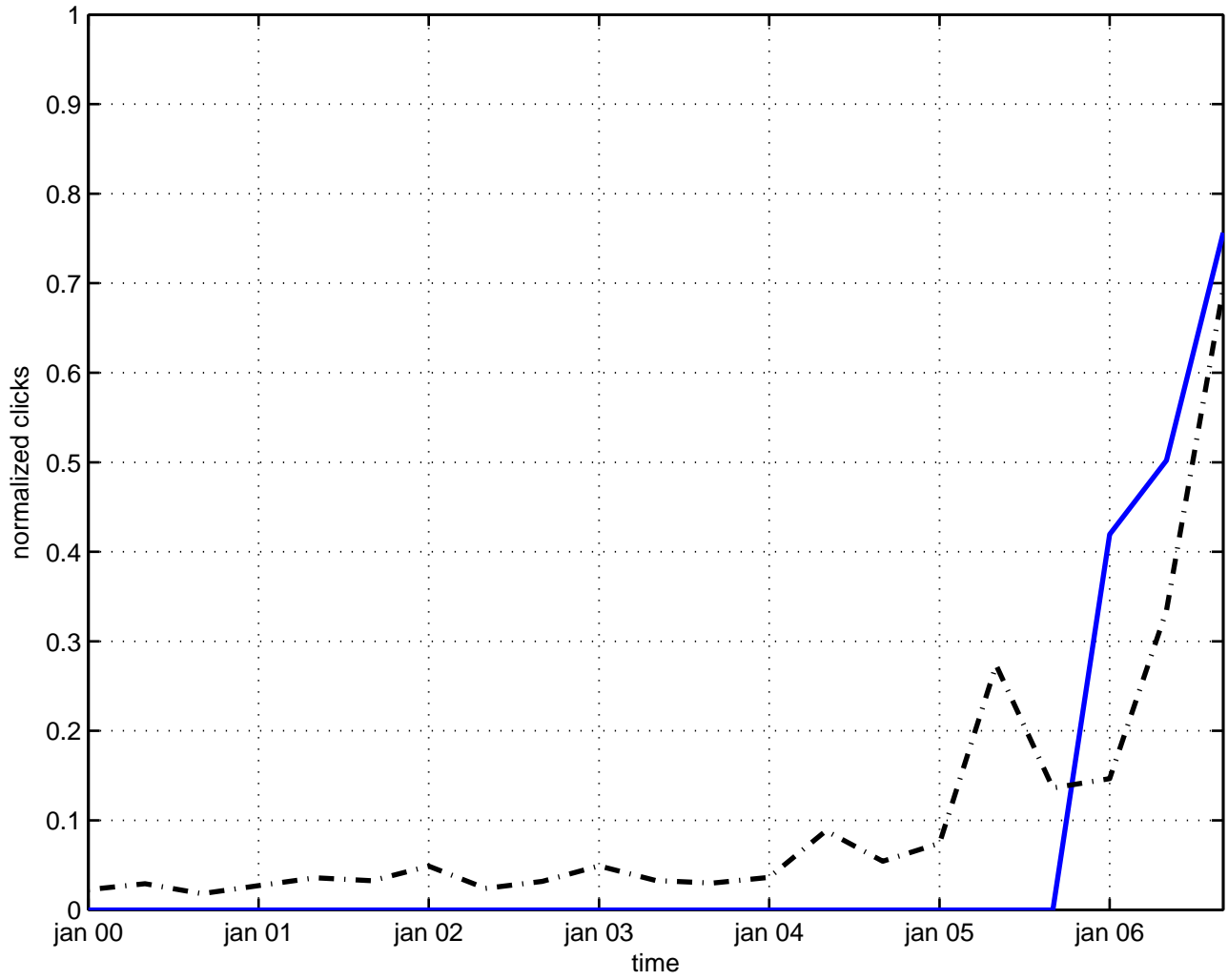
localization fermion
