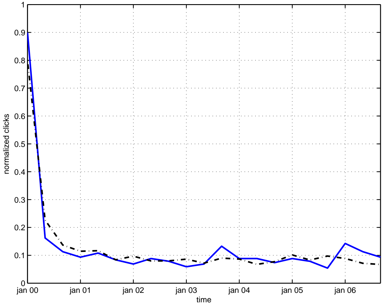
local s-matrix
