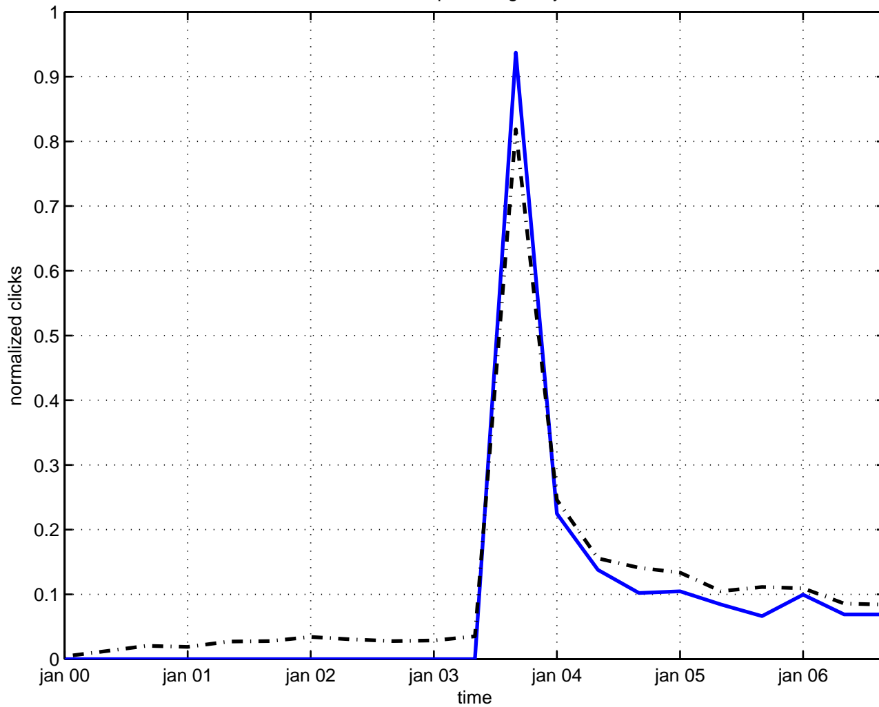
local quantum gravity
