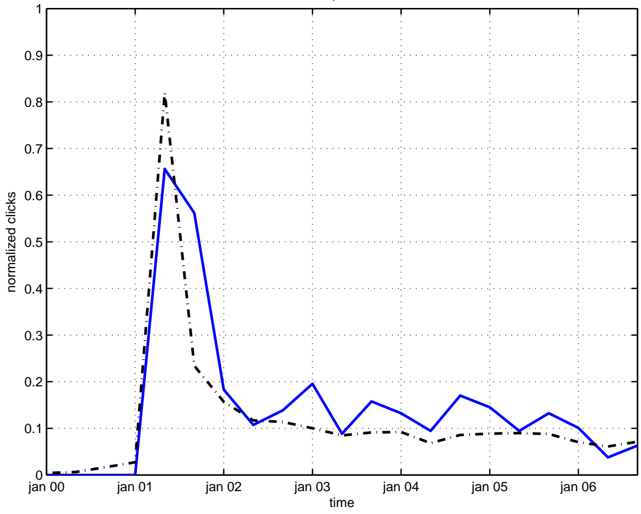
local potential
