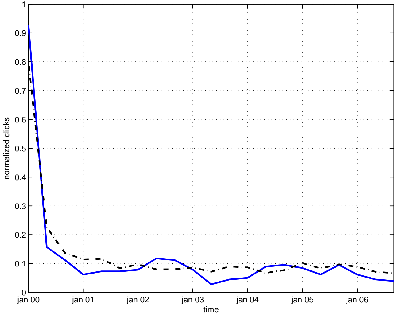
local perturbation theory
