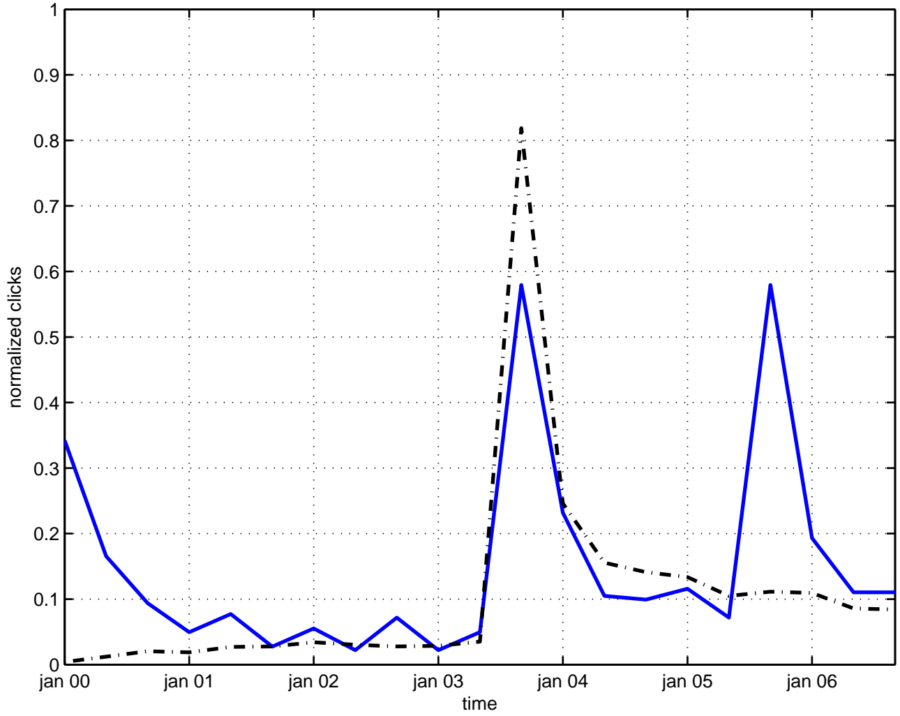
liquid instanton
