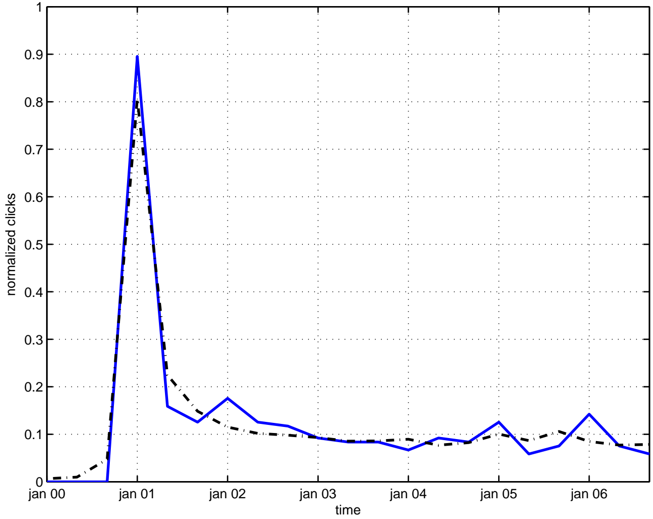
lippmann-schwinger equation
