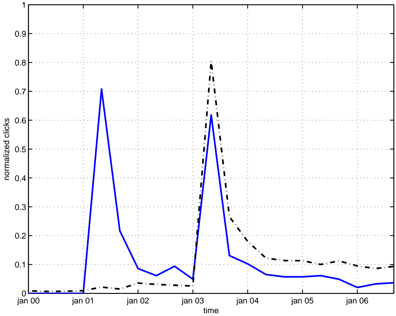
liouville string model
