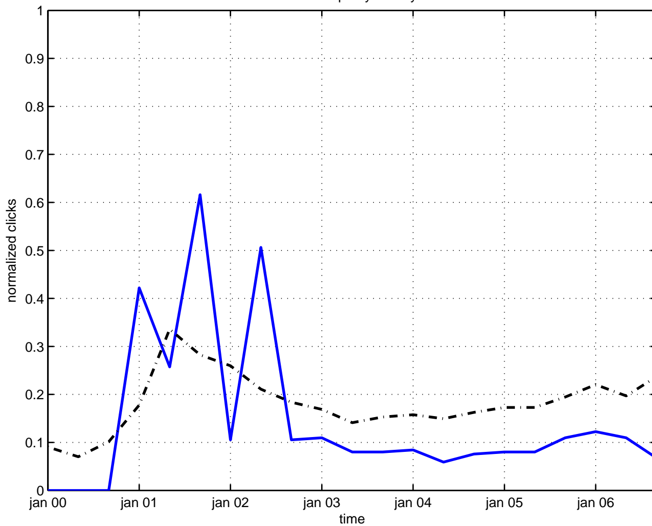
linear supersymmetry
