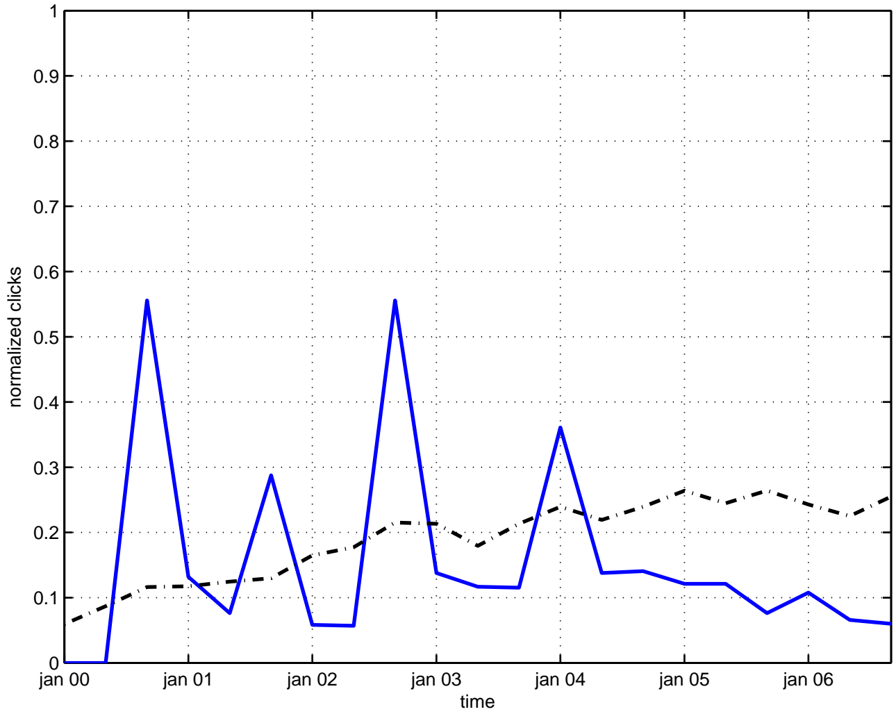
linear supergravity
