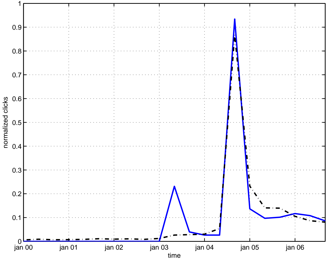
linear stability
