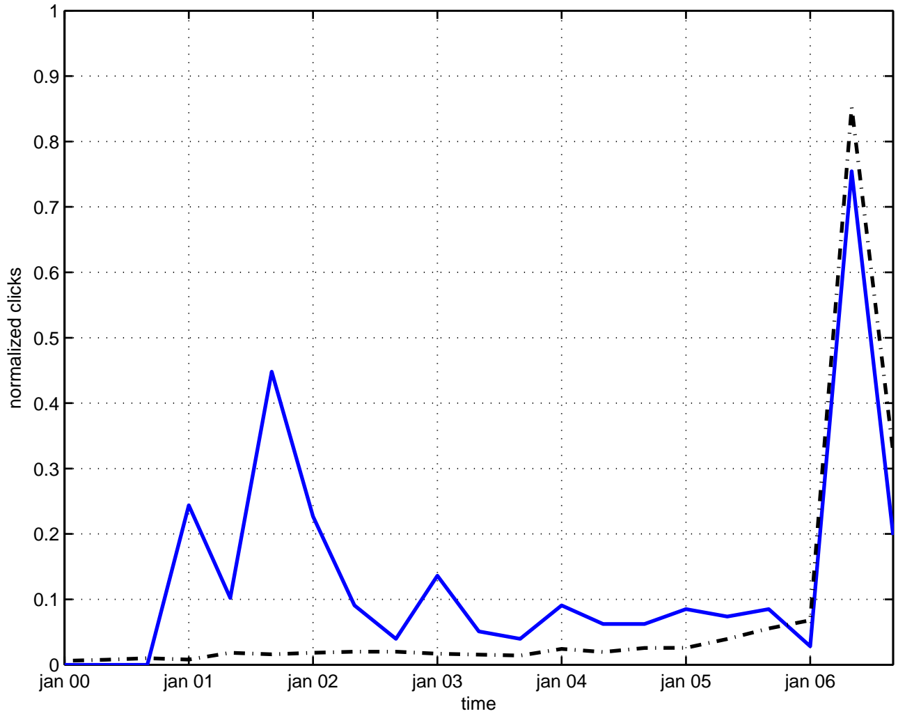
linear constraint
