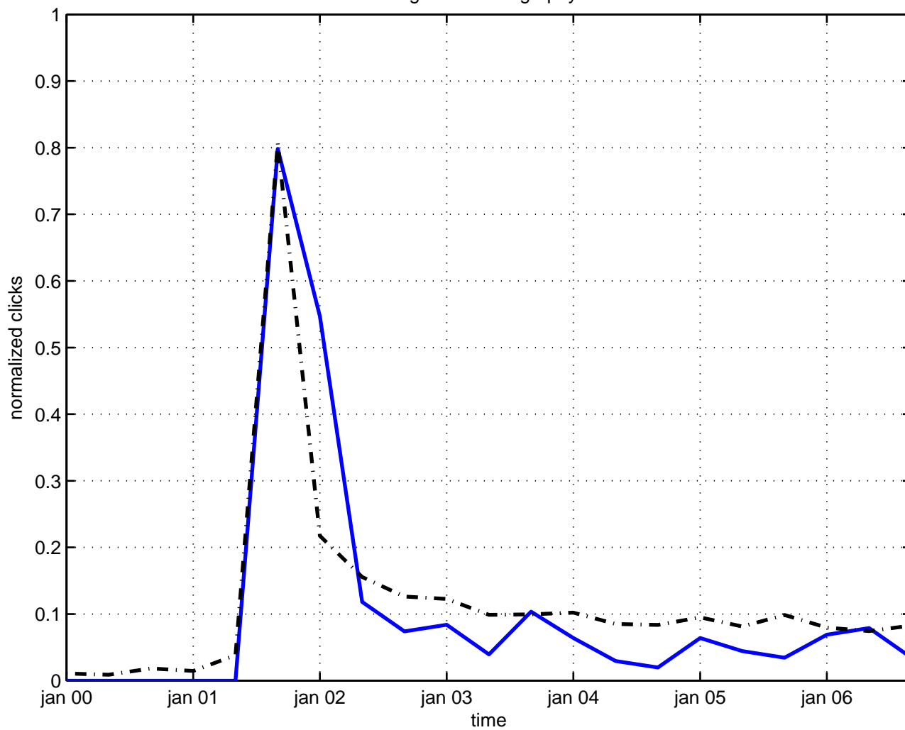
light front holography
