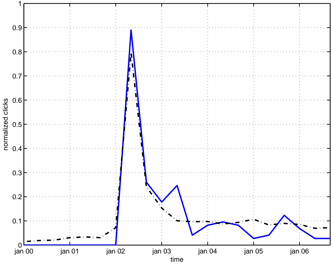
light front field theory
