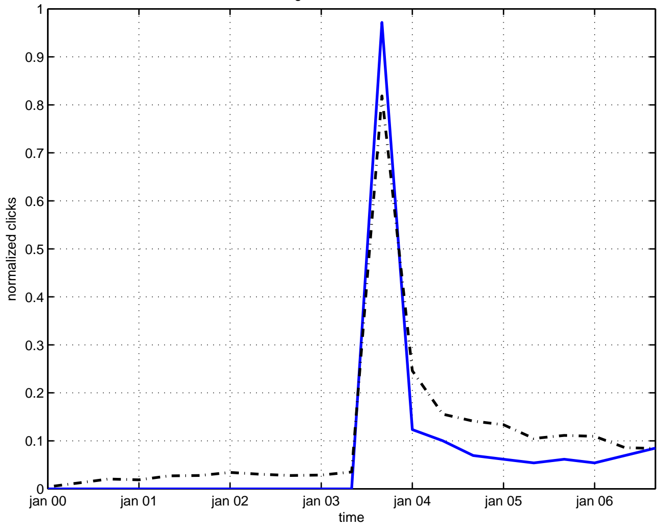
light cone zero mode
