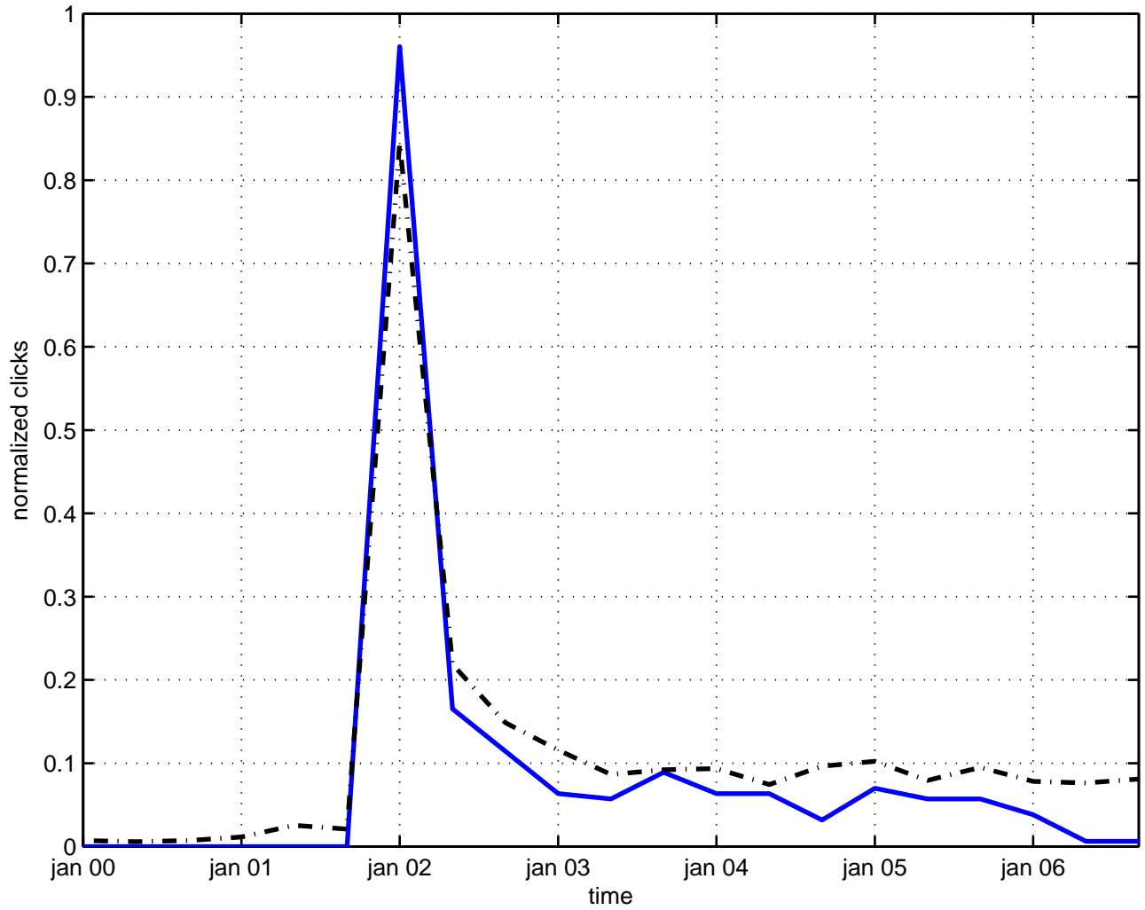
light cone supersymmetry
